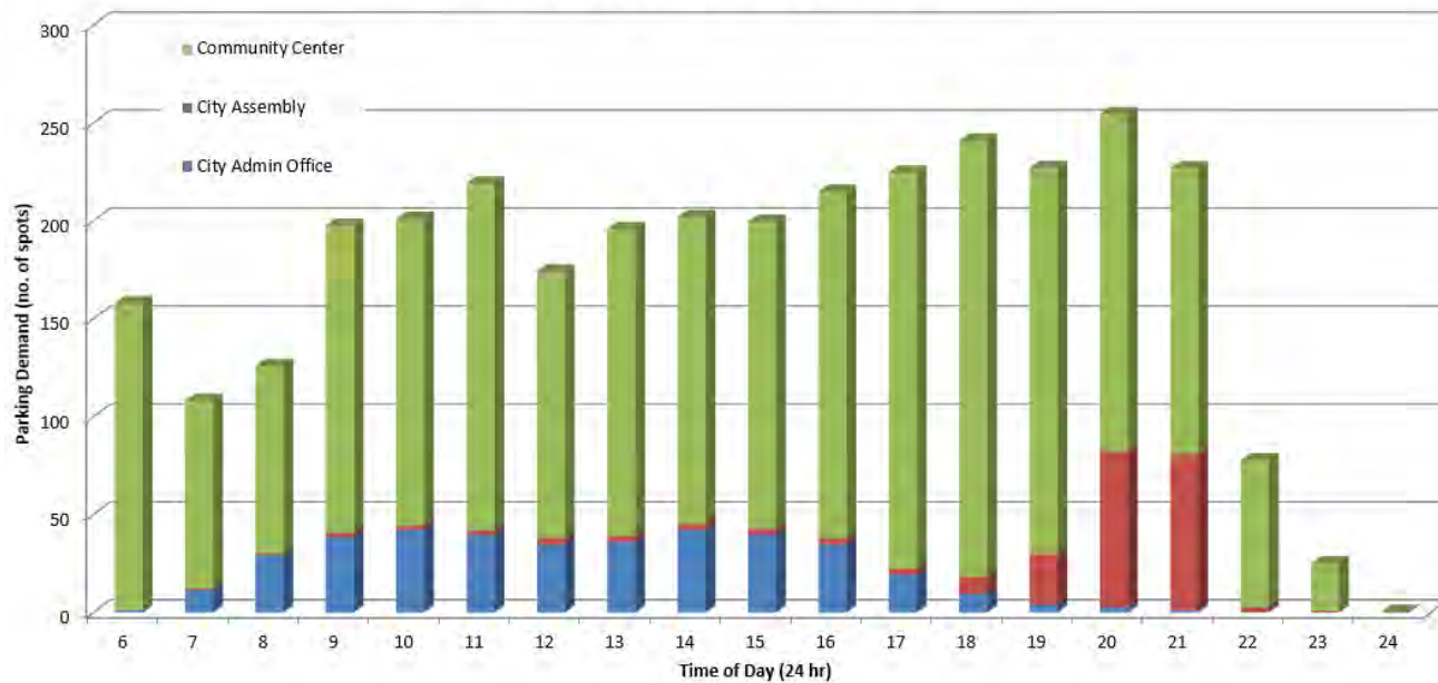
Adjusted JAN Weekday Parking Demand
