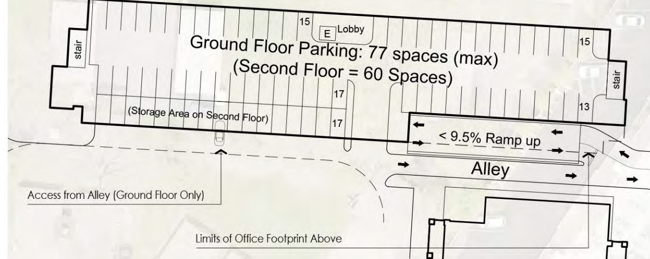
Parking Under Mixed-Use Building (NTS)
